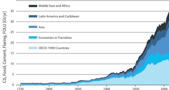
Figure 1: Annual Release of CO 2 into the Atmosphere (IPCC, 2021)
